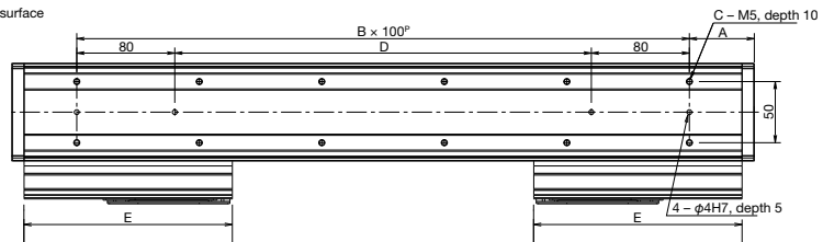
Cable track for user wiring (type M)
