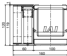
Cable track for user wiring (type S)
